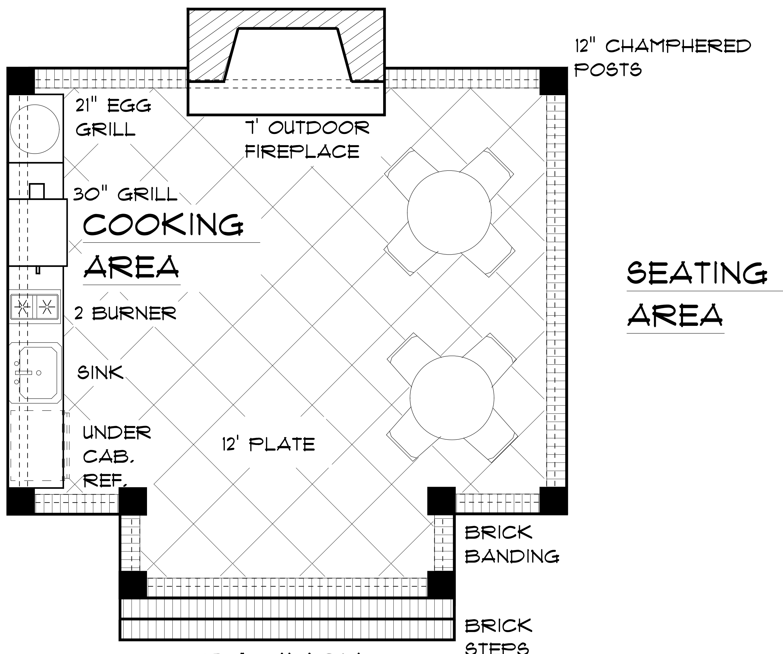
PAVILION FLOOR PLAN
